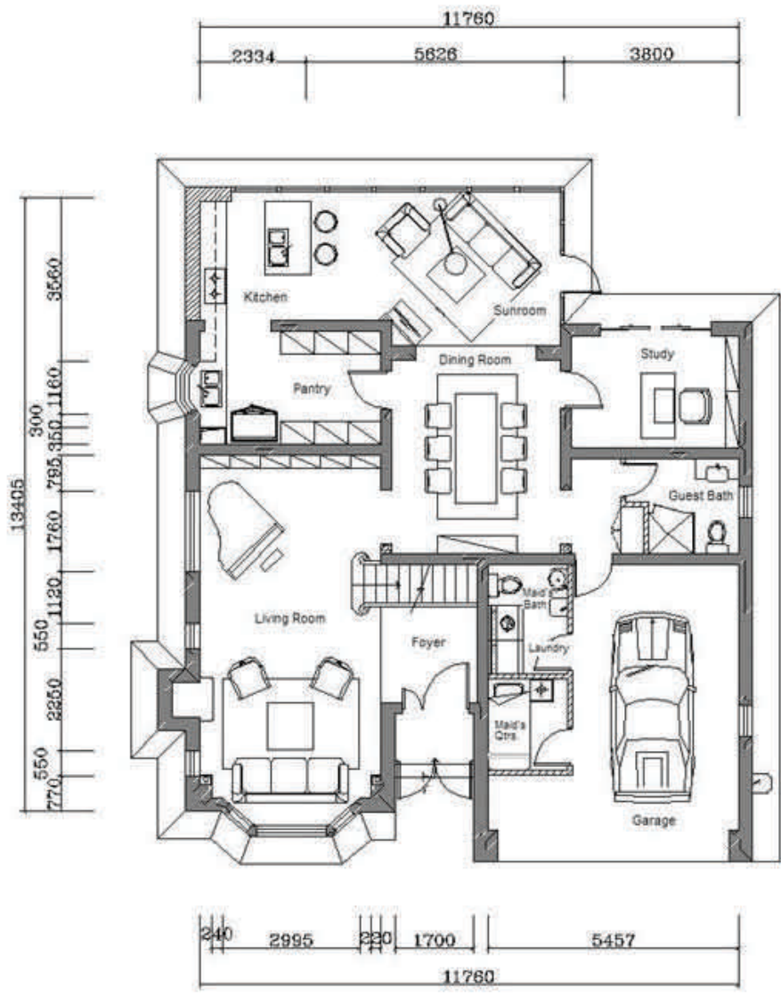
1F First Floor Plan Scale 1:100
