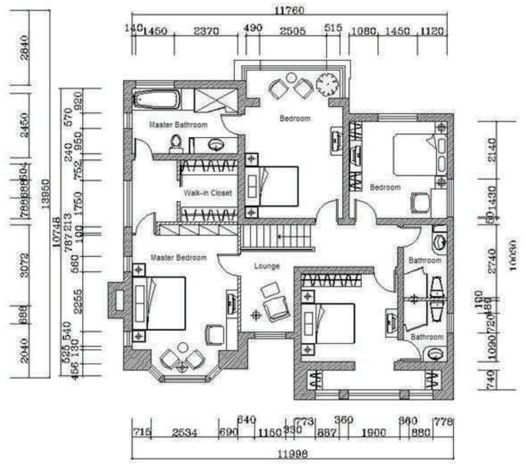
2F Second Floor Plan Scale 1:100
